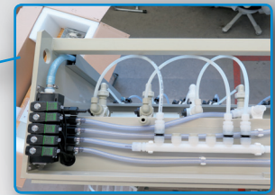
Integrated manifold
